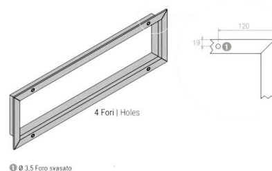
4 Fori | Holes Ø 3.5 Foro svasato
